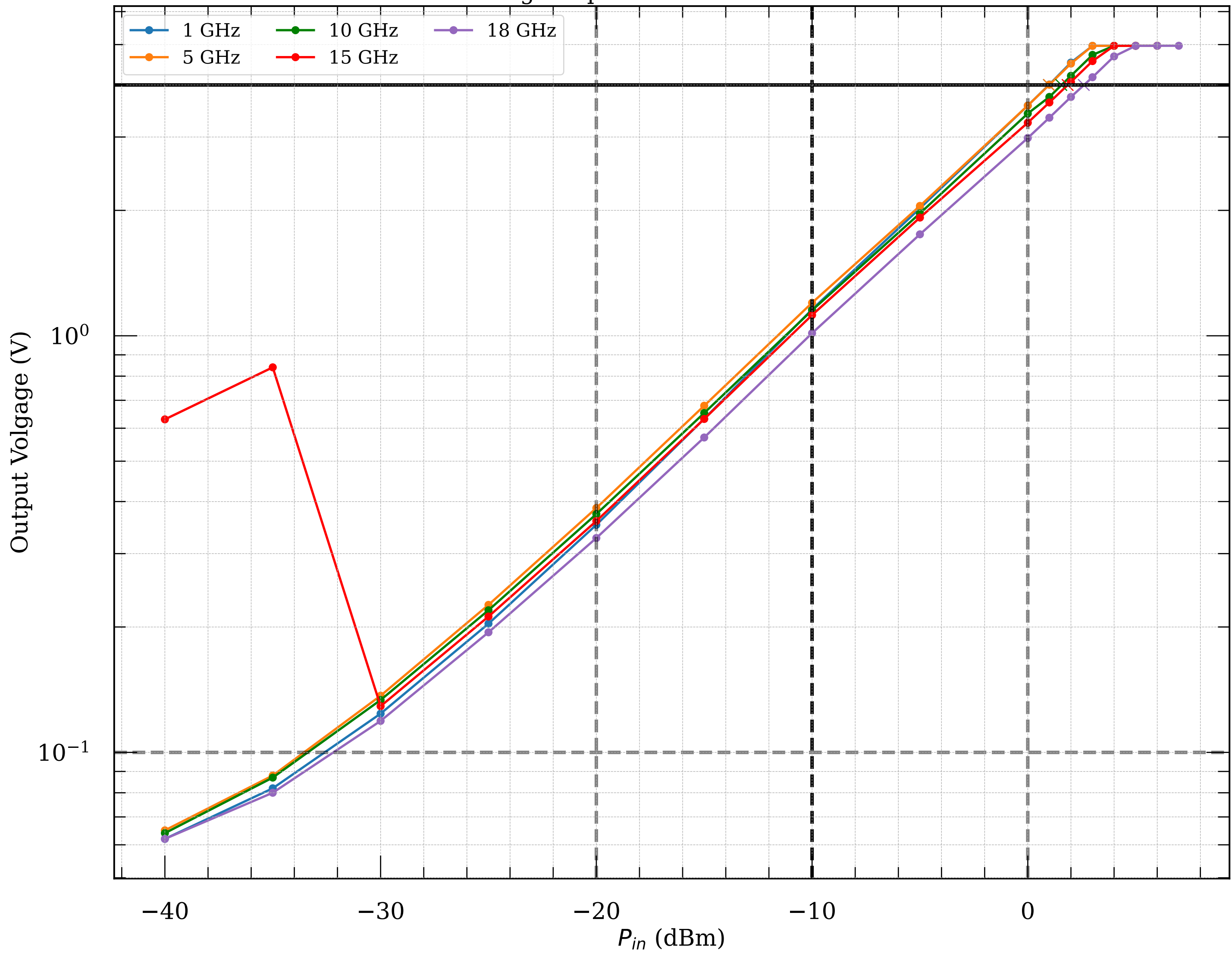
Measured voltage-to-power curve of detector module095
